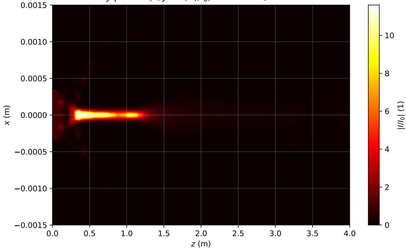
Intensity profile I(x, y = 0, z)/I_0 , P_{in}=6.0P_{cr} , artificial time
